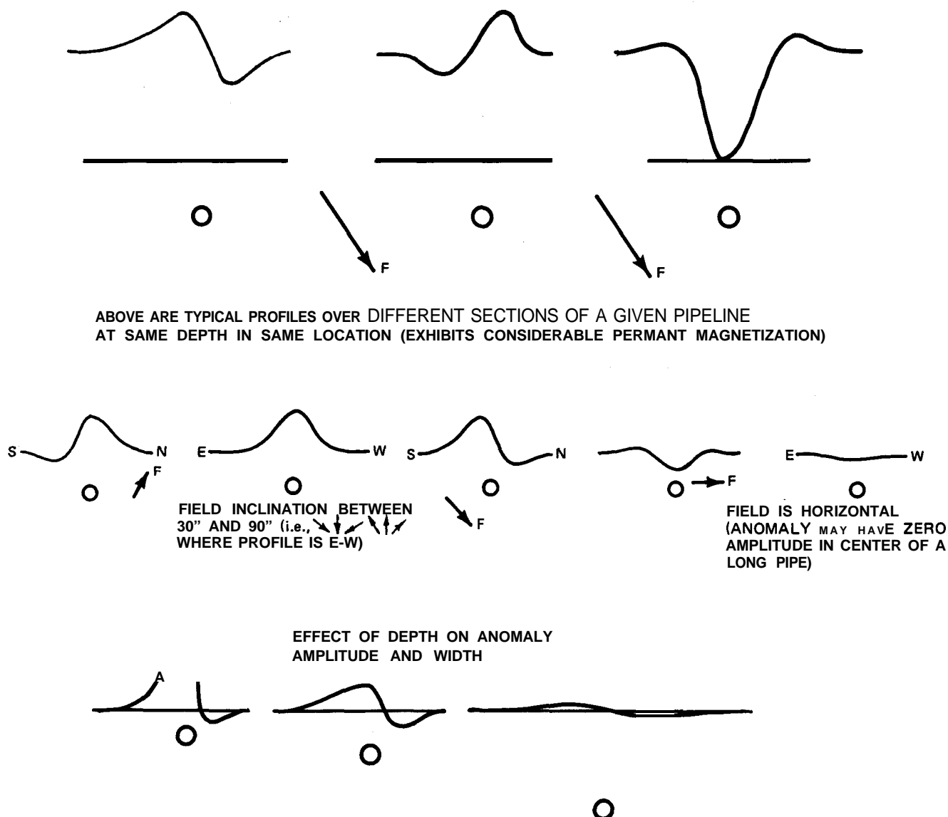
Figure 47. Pipeline Signatures
