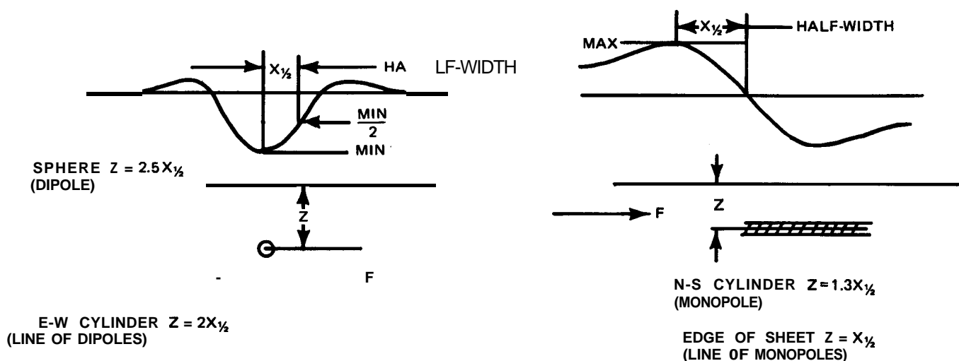
Figure 36. Half-width Rules - Horizontal Field (Equatorial)
