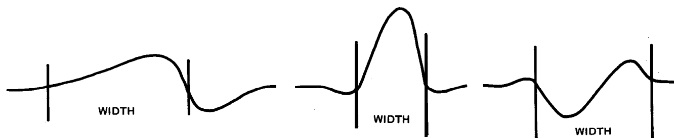
Figure 33. Anomaly 'Width'
