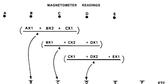
Figure 9. Profile Smoothing
